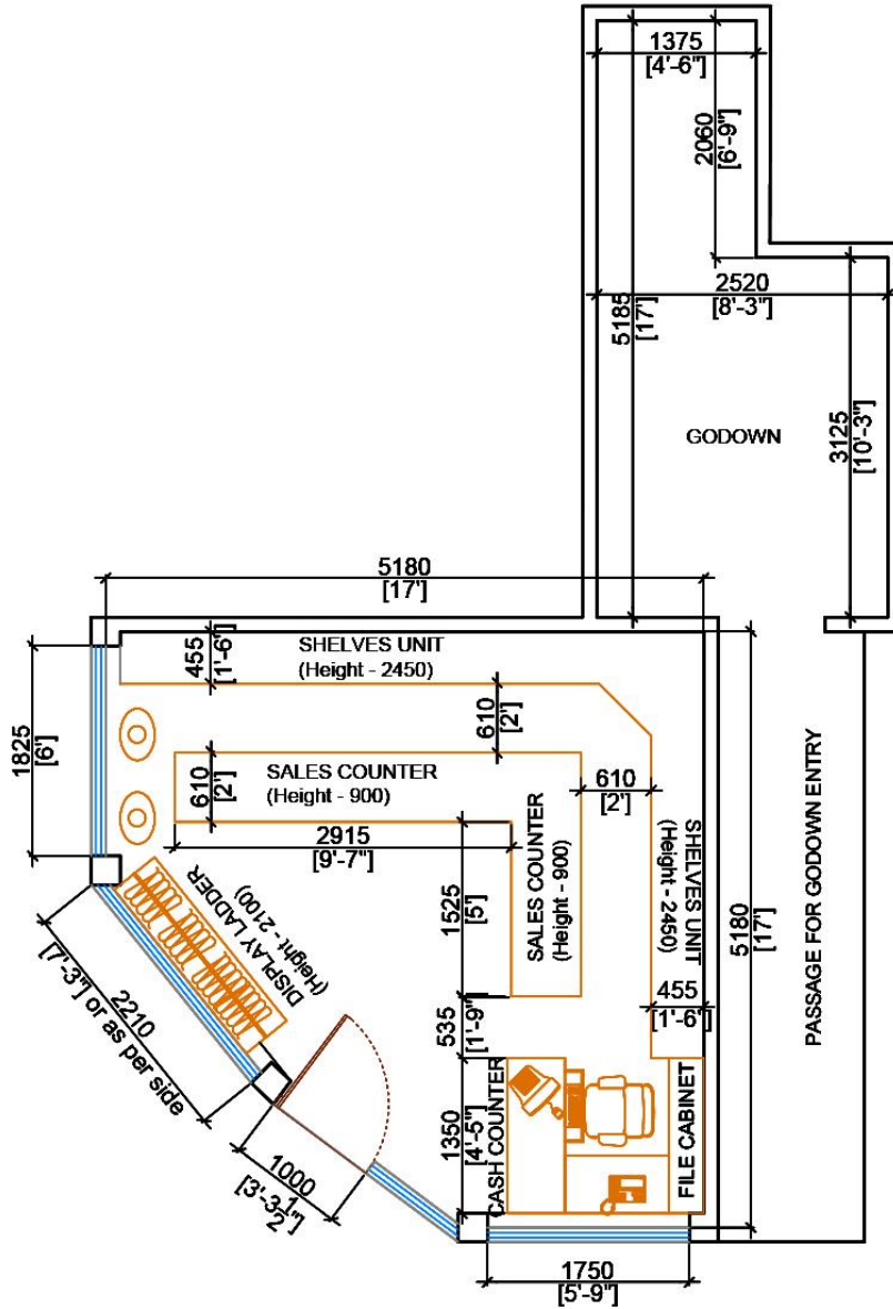
FLOOR LAYOUT PLAN
