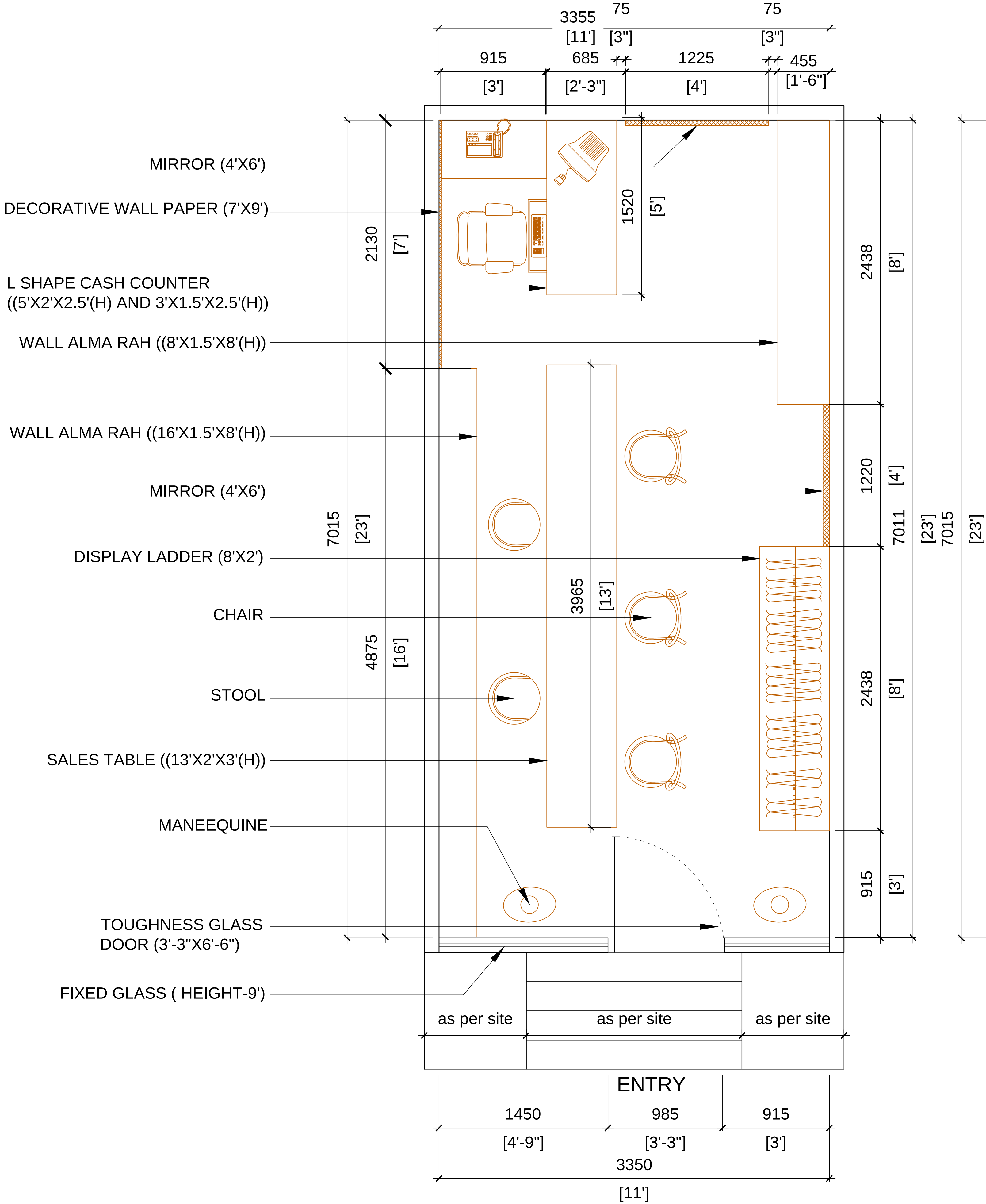
FLOOR LAYOUT PLAN
